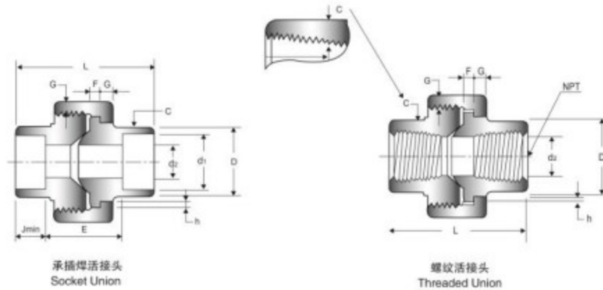
承插焊和螺纹活接头 Unions of Socket-Welding & Threaded MSS SP-83
